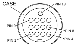
13 PIN FEMALE MATING FACE
