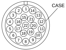
22 PIN MALE MATING FACE
